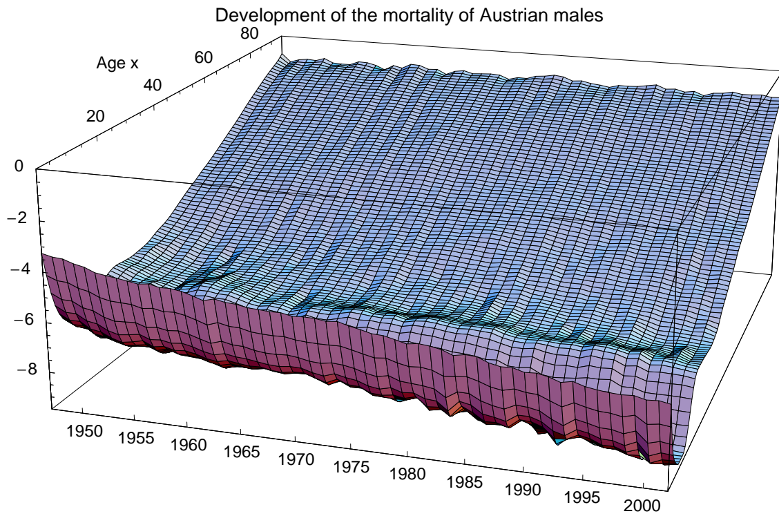
Figure 5: Logarithm of the yearly mortality of Austrian males since 1947.
