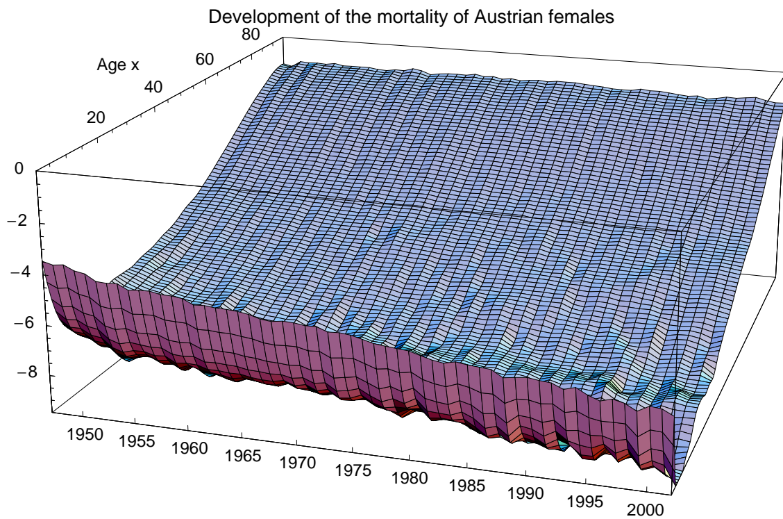
Figure 6: Logarithm of the yearly mortality of Austrian females since 1947.
